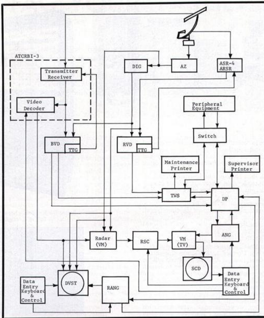
figure 2—functional element block diagram
